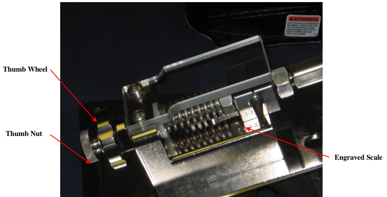
Figure 1: Jaw Adjustment
