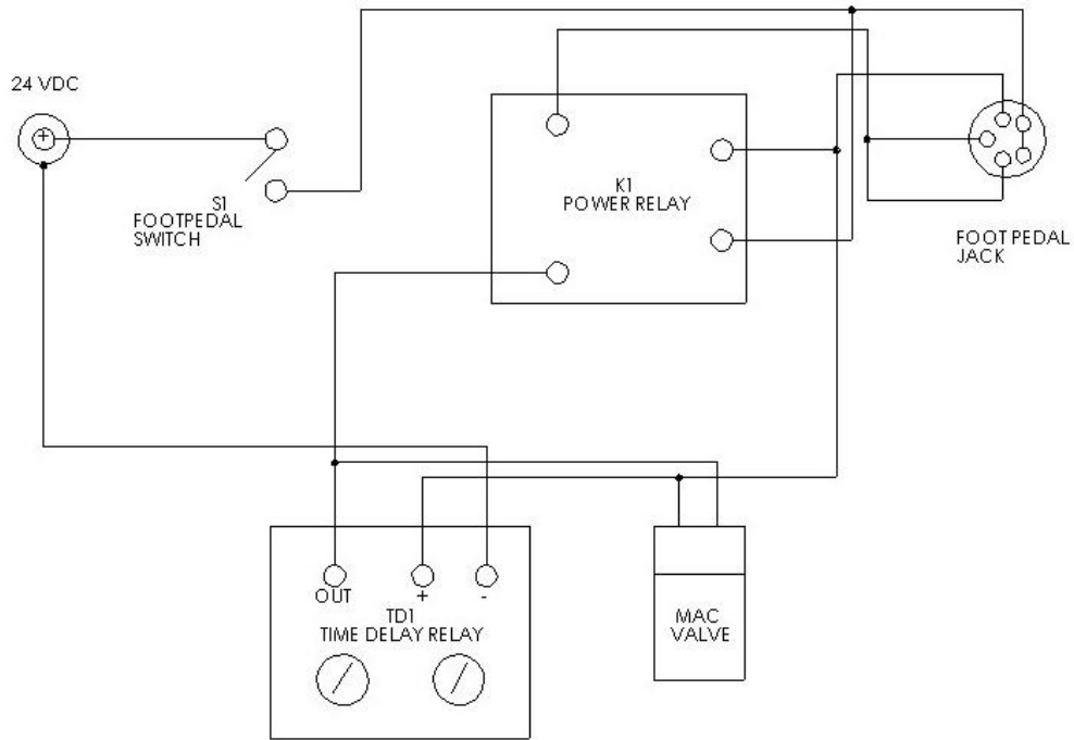
WIRING DIAGRAM CRD 201 TD EXPANDER
